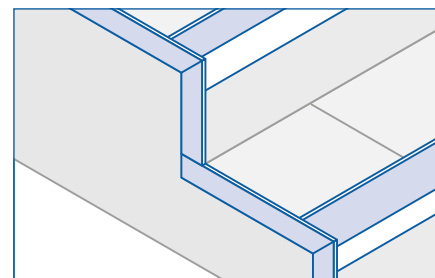
TA5 welded corner providing a flush, neat finish to a BASICZ stair edging profile.
